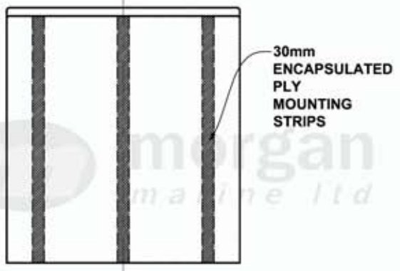
EXTERNAL VIEW WALL 3
