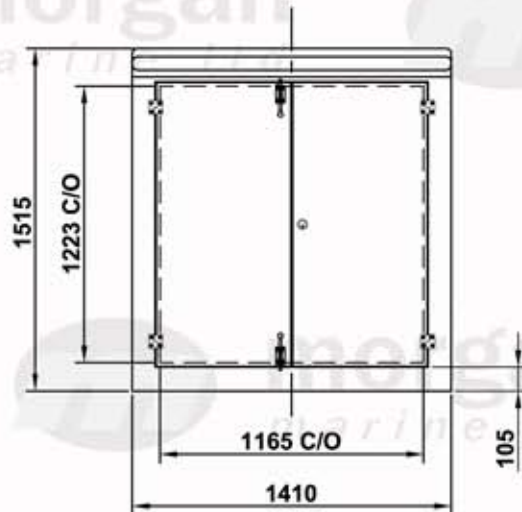
EXTERNAL VIEW WALL 1
