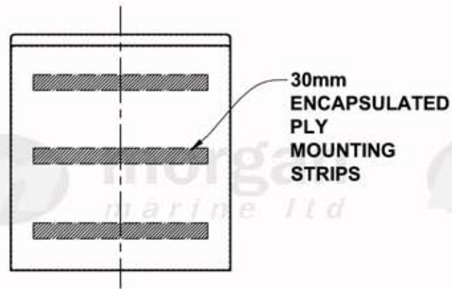
EXTERNAL VIEW WALL 3
