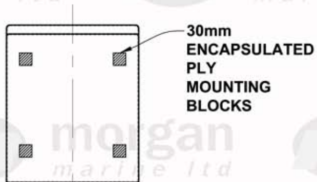
EXTERNAL VIEW WALL 3
