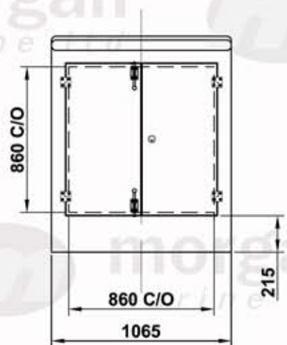
EXTERNAL VIEW WALL 1
